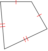
kite
