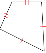
kite
