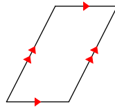
parallelogram
