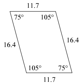
parallelogram
