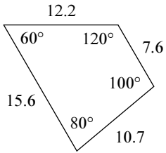
trapezoid
