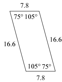
parallelogram
