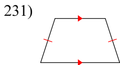
isosceles trapezoid
