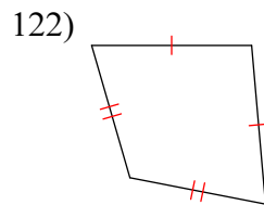
kite
