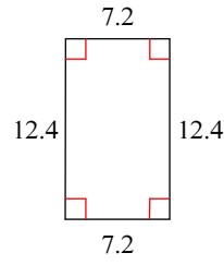
rectangle
