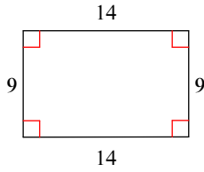
rectangle
