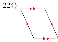
parallelogram
