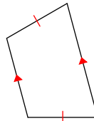
isosceles trapezoid
