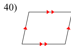
parallelogram
