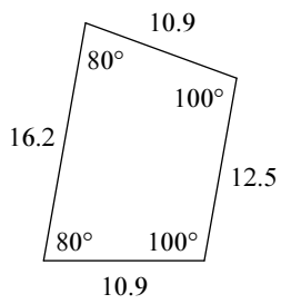
isosceles trapezoid
