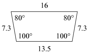
isosceles trapezoid
