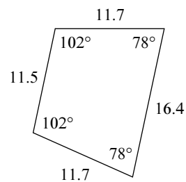
isosceles trapezoid
