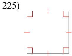
square
