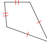
kite
