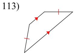
isosceles trapezoid
