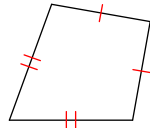
kite
