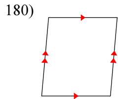
parallelogram
