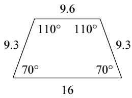
isosceles trapezoid
