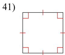
square
