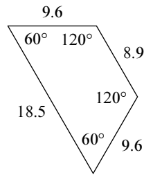
isosceles trapezoid
