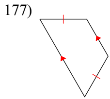
isosceles trapezoid
