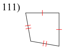
kite
