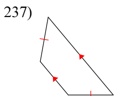
isosceles trapezoid
