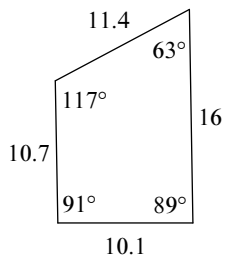
trapezoid
