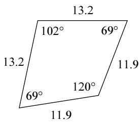
kite
