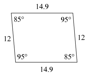
parallelogram
