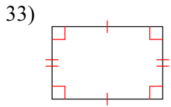
rectangle
