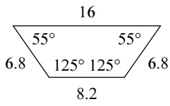
isosceles trapezoid
