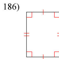
rectangle
