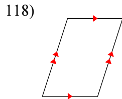
parallelogram
