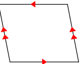
parallelogram
