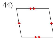
parallelogram
