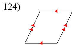
parallelogram
