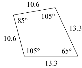
kite
