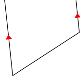
trapezoid
