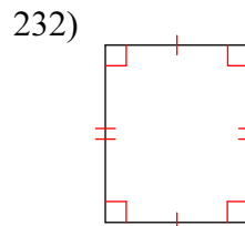
rectangle
