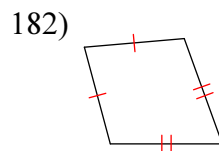
kite
