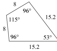
kite
