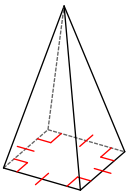
square pyramid
