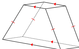
trapezoidal prism
