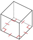
square prism
