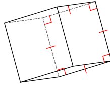
square prism
