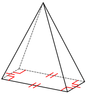
rectangular pyramid
