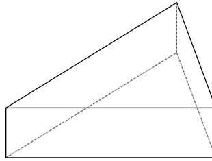
triangular prism
