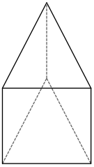
triangular prism
