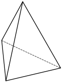
triangular pyramid
