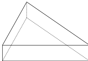
triangular prism
