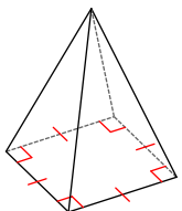
square pyramid
