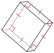
square prism
