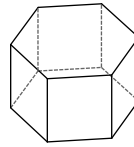
hexagonal prism
