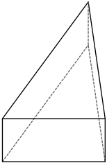
triangular prism
