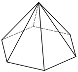
hexagonal pyramid
