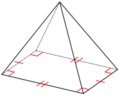
rectangular pyramid
