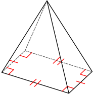
rectangular pyramid
