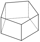
pentagonal prism
