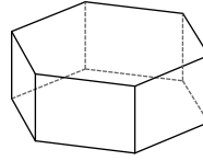
hexagonal prism
