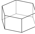
hexagonal prism
