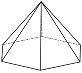
hexagonal pyramid
