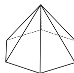
hexagonal pyramid
