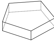
pentagonal prism
