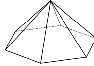
hexagonal pyramid
