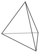
triangular pyramid
