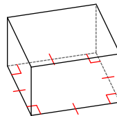
square prism
