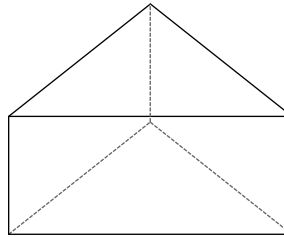
triangular prism
