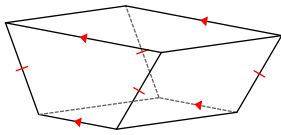
trapezoidal prism
