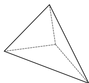
triangular pyramid
