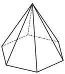
hexagonal pyramid
