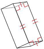
rectangular prism
