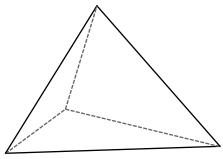
triangular pyramid
