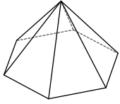
hexagonal pyramid
