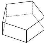
pentagonal prism
