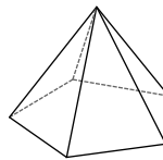
pentagonal pyramid
