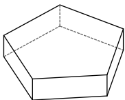
pentagonal prism
