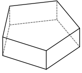
pentagonal prism
