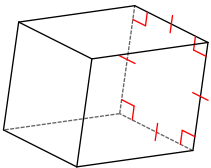
square prism
