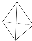
triangular pyramid
