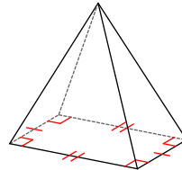
rectangular pyramid
