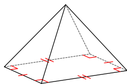
rectangular pyramid
