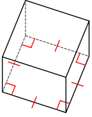
square prism
