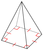
square pyramid
