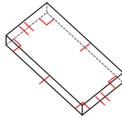
rectangular prism
