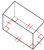
rectangular prism
