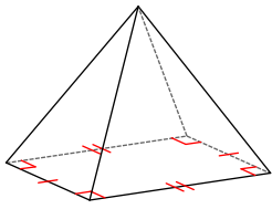
rectangular pyramid
