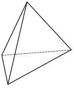
triangular pyramid
