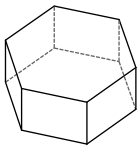
hexagonal prism
