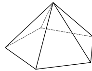
pentagonal pyramid
