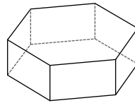
hexagonal prism
