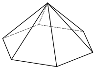
hexagonal pyramid
