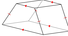
trapezoidal prism
