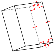
rectangular prism
