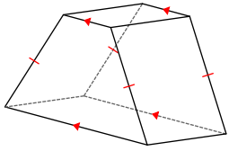
trapezoidal prism
