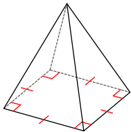
square pyramid
