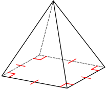
square pyramid
