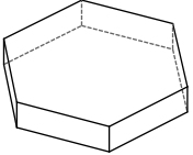
hexagonal prism
