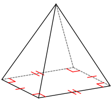
rectangular pyramid
