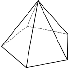
pentagonal pyramid
