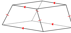
trapezoidal prism
