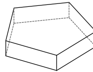
pentagonal prism
