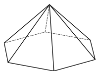
hexagonal pyramid
