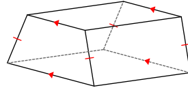
trapezoidal prism
