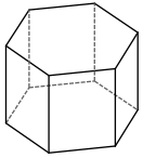
hexagonal prism
