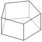
pentagonal prism
