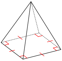
square pyramid
