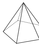
pentagonal pyramid
