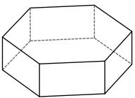
hexagonal prism
