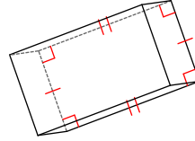
rectangular prism
