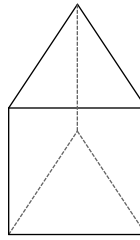
triangular prism
