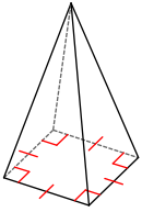
square pyramid
