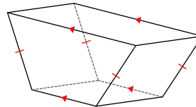
trapezoidal prism
