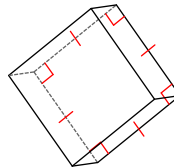
square prism
