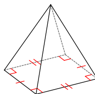
rectangular pyramid
