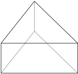
triangular prism
