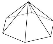
hexagonal pyramid
