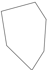
hexagon
