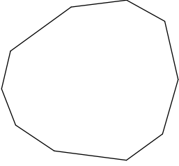
decagon
