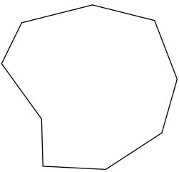
nonagon
