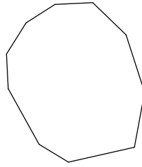
decagon
