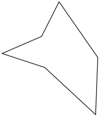
hexagon
