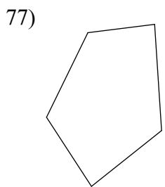
pentagon
