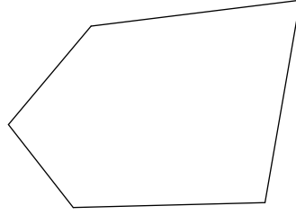
pentagon
