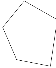
pentagon
