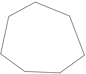
heptagon
