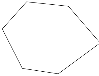
hexagon
