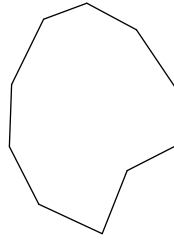
decagon
