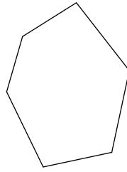
hexagon
