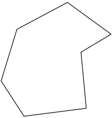
heptagon
