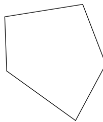
pentagon
