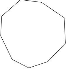
nonagon
