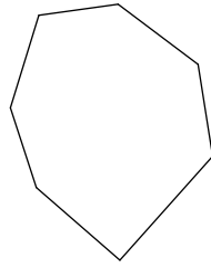
heptagon
