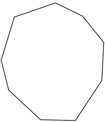
nonagon
