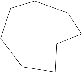
octagon
