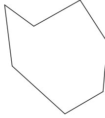
heptagon
