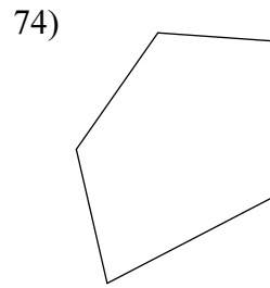
pentagon
