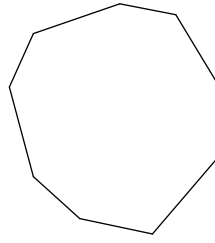
nonagon
