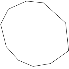
decagon
