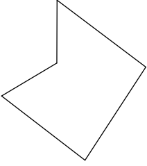
pentagon
