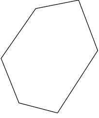
hexagon
