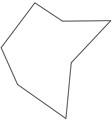
heptagon
