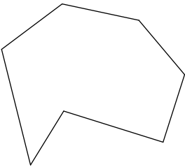
heptagon
