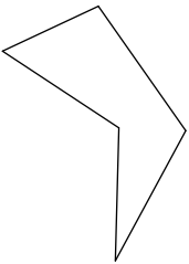
pentagon
