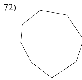
octagon
