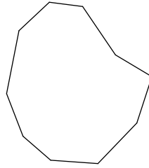
decagon
