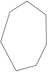
heptagon
