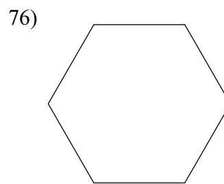
hexagon
