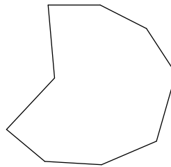
nonagon
