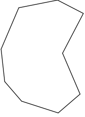
nonagon
