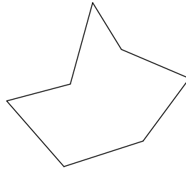
heptagon
