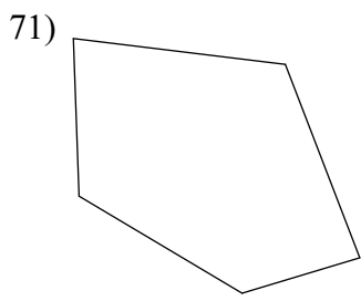
pentagon
