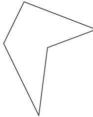
pentagon
