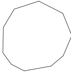
decagon
