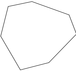
heptagon
