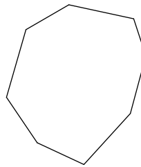
octagon
