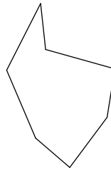
heptagon
